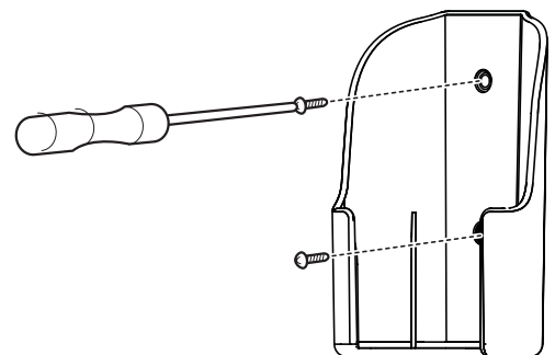
Figure 6: Holder Attachment
