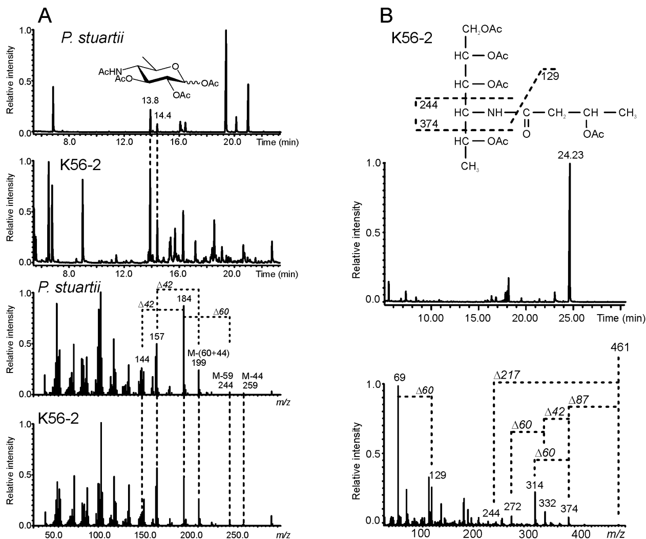
FIGURE 4. GC/MS spectra after methanolysis and \beta -elimination of B. cenocepacia FliC glycan (K56-2) and control sample (O antigen of P. stuartii O43). A, the top two graphs correspond to an overview of entire spectra for P. stuartii O43 O antigen and B. cenocepacia K56-2 FliC samples. Qui4N peaks at 13.8 and 14.4 (representing \alpha and \beta -configured derivatives) are indicated. Additional peaks detected in the O43 spectrum represent other sugars from the O antigen (44). Additional peaks in the FliC spectrum represent derivatized amino acids released from the FliC protein during methanolysis. The lower two spectra show the characteristic fragmentation pattern of ions at 13.8 min (fragmentation pattern of ion at 14.4 min was identical). M corresponds to molecular weight of derivatized Qui4N (303 Da). B, the top graph shows an overview of the GC spectrum of the glycan released from FliC during \beta -elimination. Insert shows the derivatized glycan (461 Da) with the characteristic fragmentation pattern of the sugar and 3-hydroxy butyric acid. Lower graph shows the MS/MS fragmentation spectrum of the ion at 24.23 min. Differences between fragment ions ( \Delta ) correspond to CH 2 CO ( \Delta 42 ), CH 3 CHO ( \Delta 44 ), CH 3 COO - ( \Delta 59 ), and CH 3 COOH ( \Delta 60 ).
